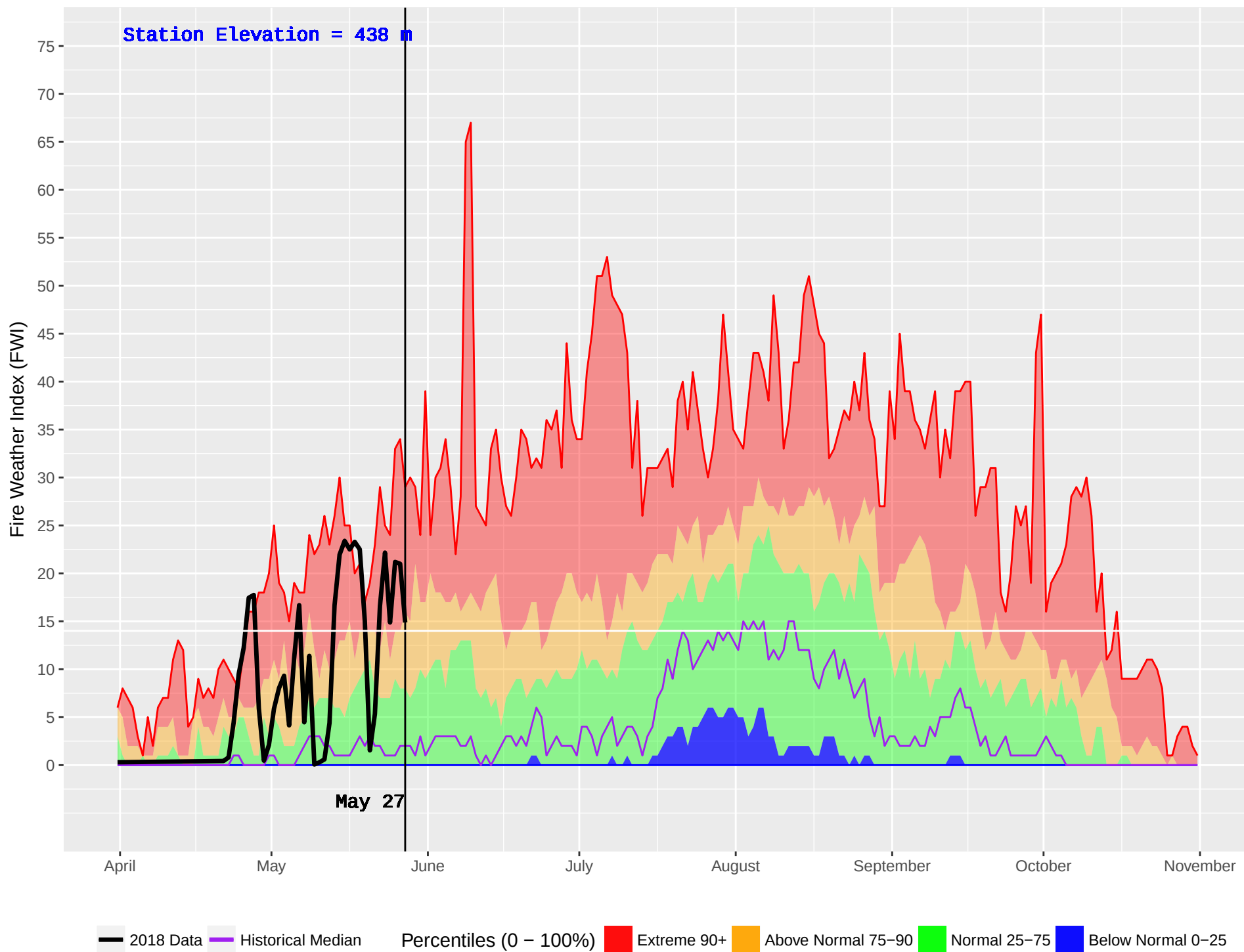
MENZIES CAMP (19) : Historical (1970–2016) and Current (2018) Noon Fire Weather Index (FWI)
