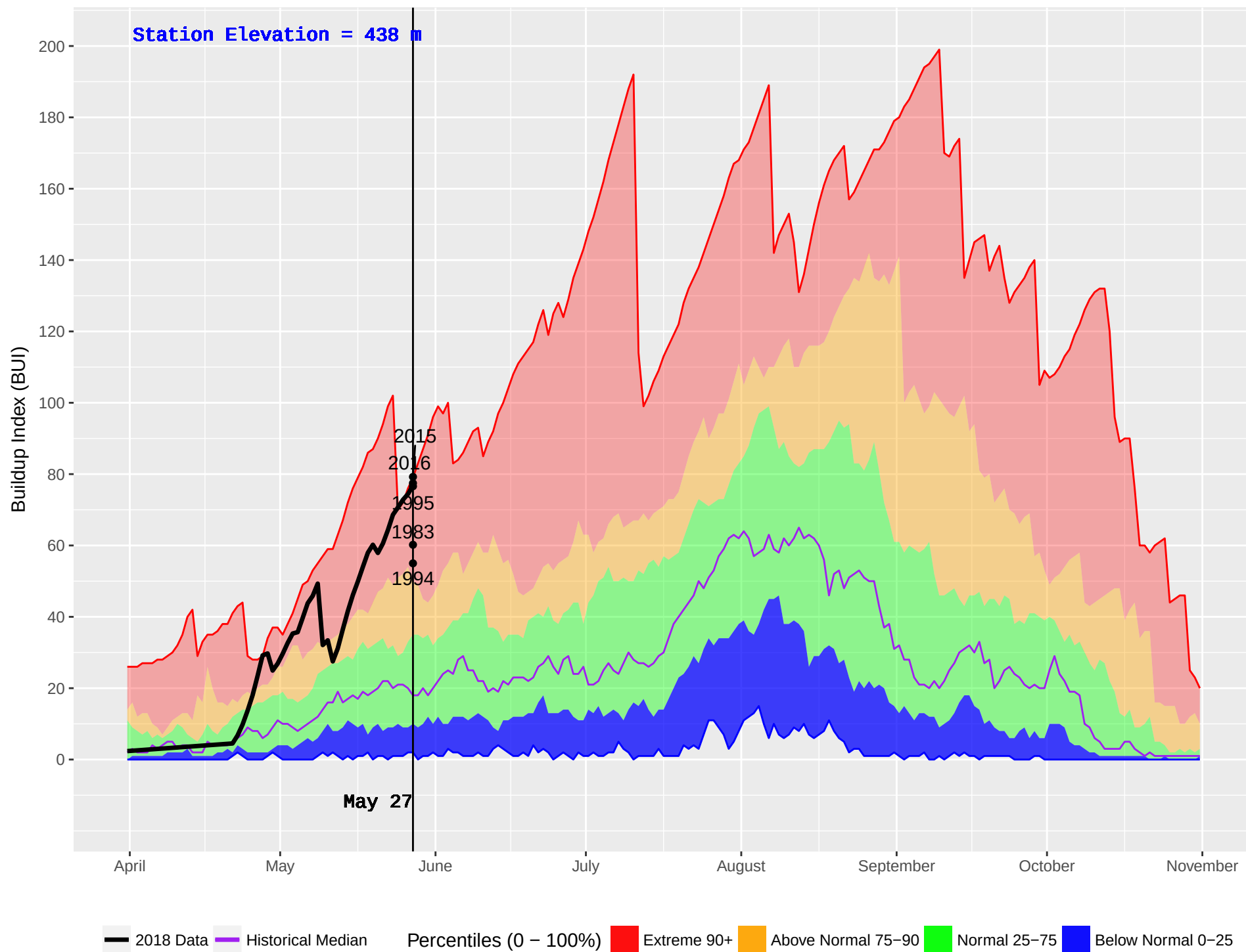
MENZIES CAMP (19) : Historical (1970–2016) and Current (2018) Noon Buildup Index (BUI)
