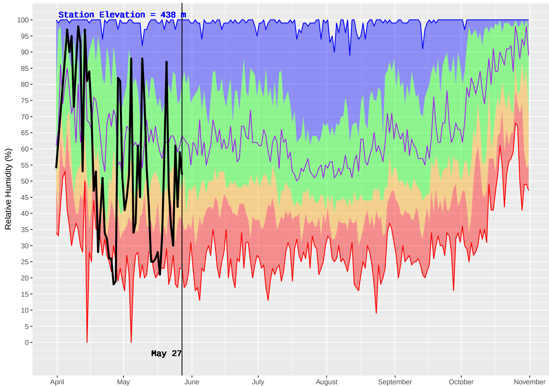
MENZIES CAMP (19) : Historical (1970–2016) and Current (2018) Noon Relative Humidity
