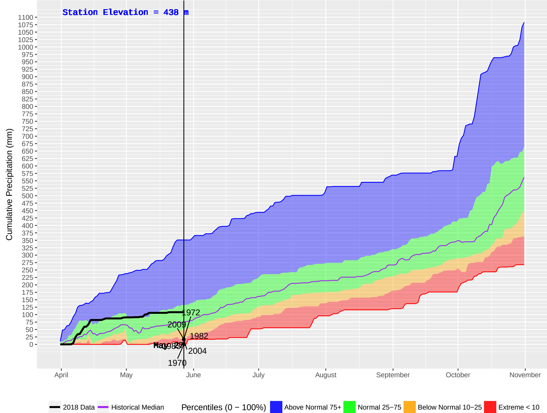
MENZIES CAMP (19) : Historical (1970–2016) and Current (2018) Noon Cumulative Precipitation
