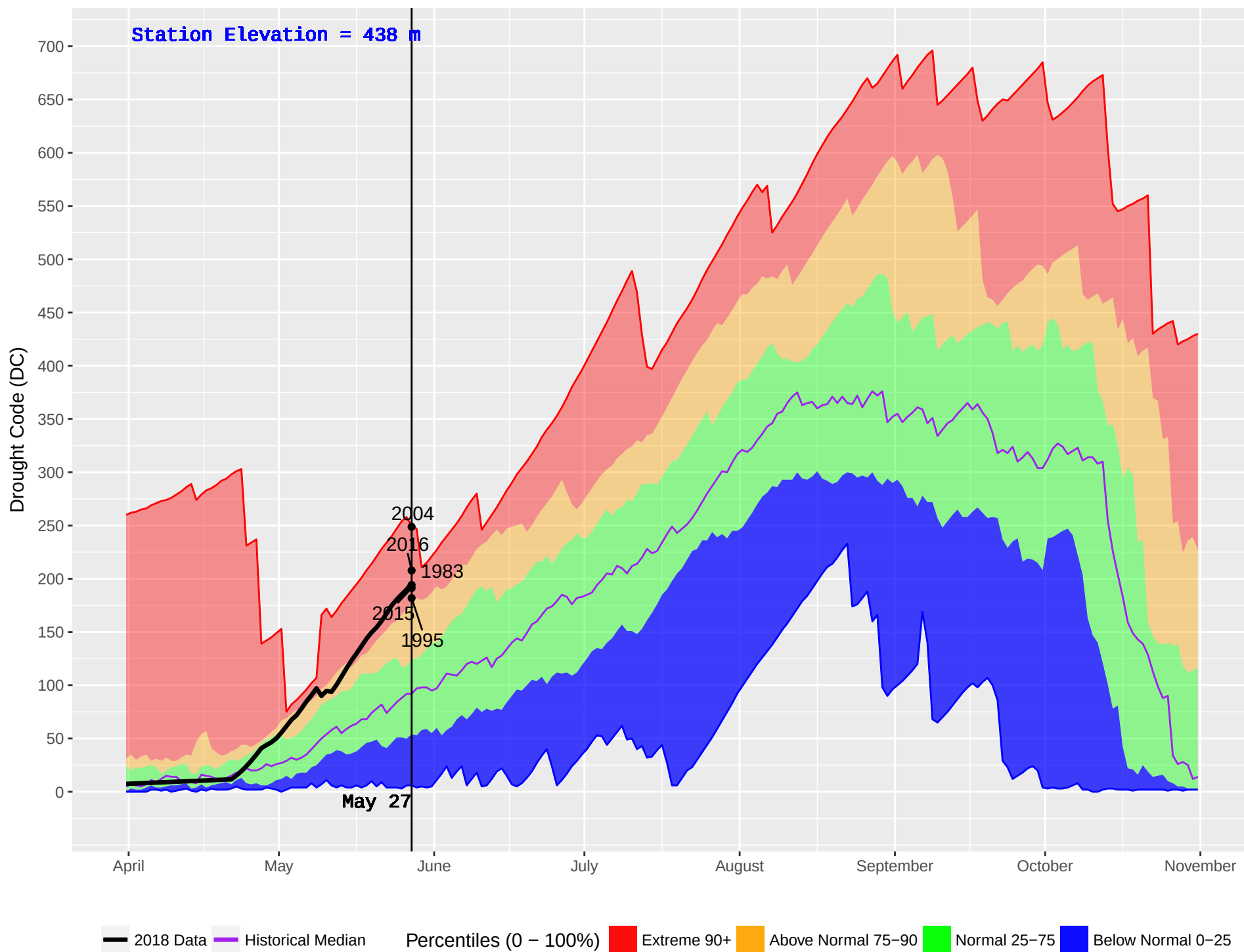
MENZIES CAMP (19) : Historical (1970–2016) and Current (2018) Noon Drought Code (DC)
