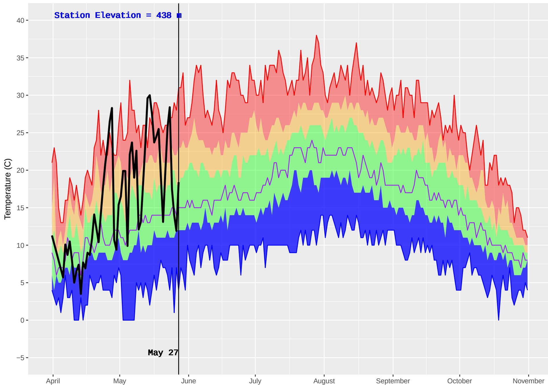
MENZIES CAMP (19) : Historical (1970–2016) and Current (2018) Noon Temperature
